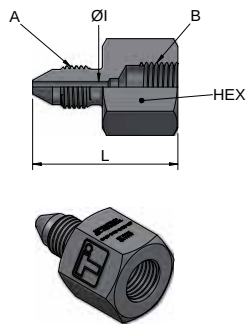
Male MP | Female GAS 120
