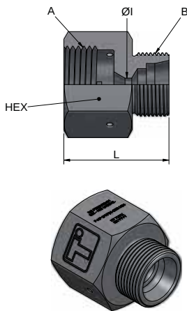
Female HP | Male CES
