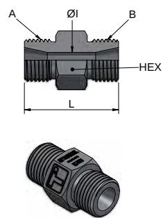
Male Metric 24/60 | Male Metric 24/60
