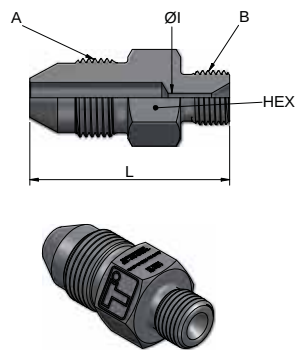
Male MP | Male Type-M
