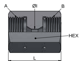
Female HP Compact (Metric Gland) | Female HP Compact (Metric Gland)
