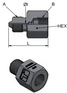
Male HP | Female GAS 120
