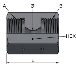
Female HP Metric Compact | Female HP Metric Compact
