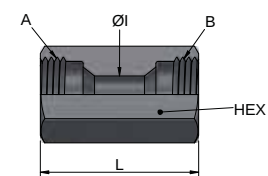
Female JIC | Female JIC
