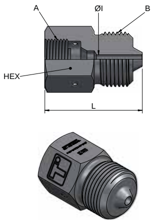
Female MP | Male HP
