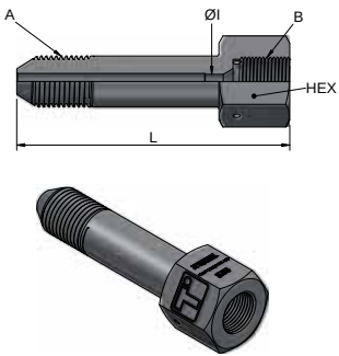
Torpedo HP | Female HP (No Gland)
